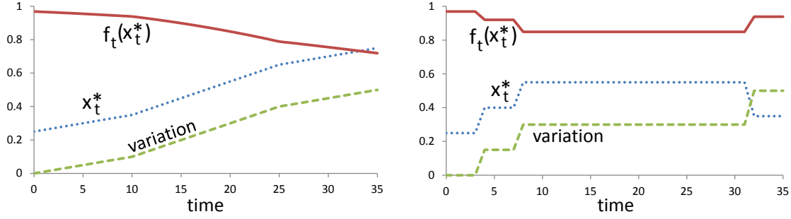
Figure 1: Variation instances within a temporal uncertainty set. Assume \mathcal{X} = [0, 1] and consider a sequence of quadratic cost functions of the form f_t(x) = \frac{1}{2}x^2 - b_t x + 1 . The change in the minimizer x_t^* = b_t , the optimal performance f_t(x_t^*) = 1 - \frac{1}{2}b_t^2 , and the variation measured by (3), is illustrated for cases characterized by continuous changes (left), and “jump” changes (right) in b_t . In both instances the variation budget is V_T = 1/2 .
