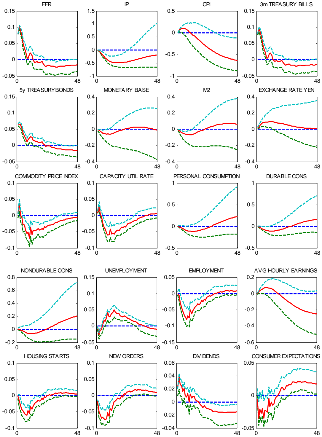
Impulse responses generated from FAVAR with 3 factors and FFR estimated by principal components with 2 step bootstrap.
