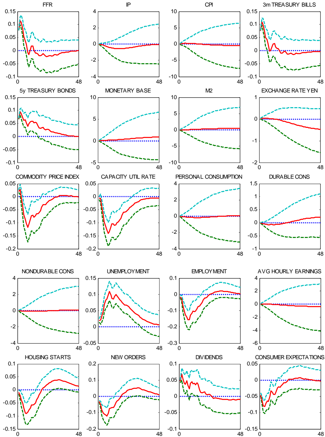
Impulse responses generated from FAVAR with 3 factors and FFR estimated by Gibbs sampling.
