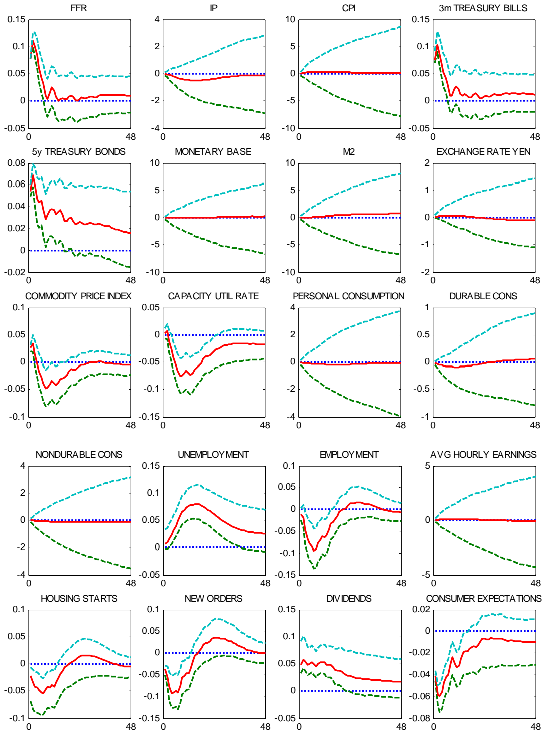
Impulse responses generated from FAVAR with 5 factors and FFR estimated by Gibbs sampling.
