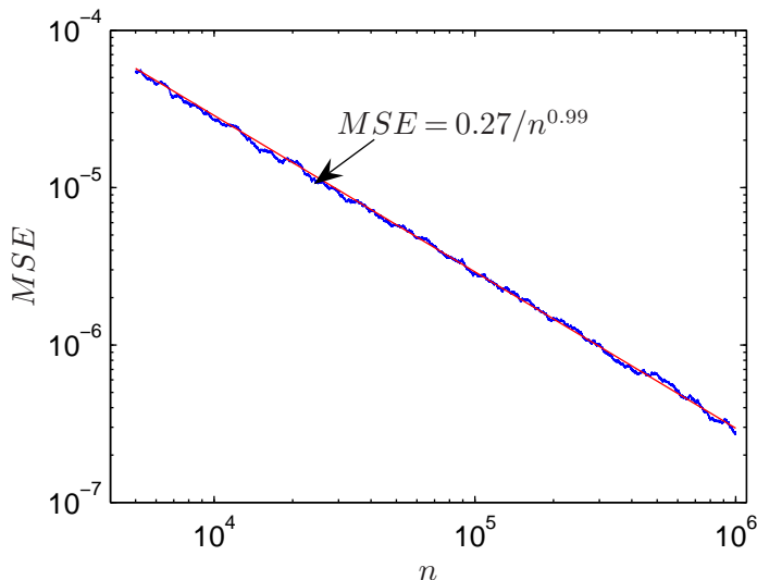
Figure 2 Illustration of non-necessity of (KW1) for “quadratic-like” functions. The log-log plot of MSE versus iteration number, n shows that the MSE behaves roughly like O(n^{-1}) which can be calculated using Proposition 2 with a_n = 1/n and c_n = 1 .
