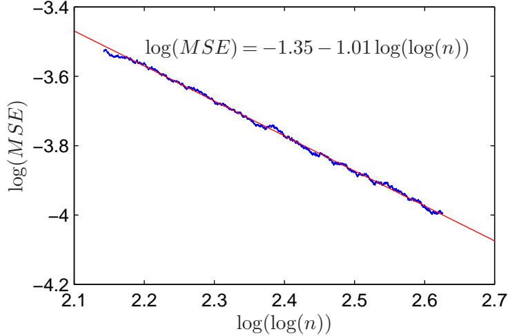
Figure 1 Illustration of the non-necessity of (KW3). The figure depicts the behavior of the MSE for a choice of sequences \{a_n\} and \{c_n\} that violates assumption (KW3); the MSE is seen to decay roughly like (\log(n))^{-1} , which follows from Theorem 1.
